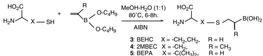
Scheme 3. Synthesis of BEHC, 3, 2MBEC, 4, and BEPA, 5.
