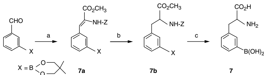
Scheme 4. Synthesis of 3-BPA 7. Reagents and conditions: (a) N -(benzyloxycarbonyl)phosphonoglycine trimethyl ester, DBU/CH 2 Cl 2 , rt, 3 h ( E/Z = 30:70); (b) 10% Pd–CH 2 /MeOH–H 2 Cl 2 (2:1), rt, 5 atm, 21 h; (c) (i) 1 M aq NaOH, 50 °C, 2 h, (ii) 2 M aq HCl, Et 2 O, PhB(OH) 2 , rt, 9 h.
