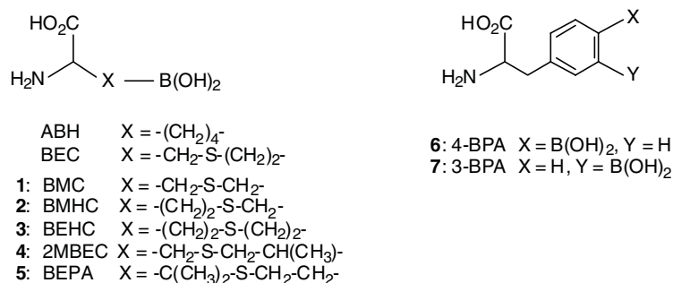
Scheme 1. Structure of ABH, BEC, and \omega -borono- \alpha -amino acids 1–7.
