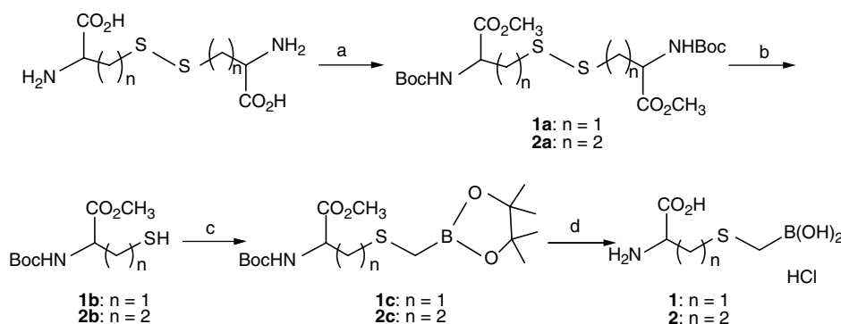
Scheme 2. Synthesis of BMC, 1 ( n = 1 ) and BMHC, 2 ( n = 2 ). Reagents and conditions: (a) (i) SOCl_2 , MeOH, reflux, 12 h; (ii) NaOH, dioxane/ H_2O (2:1) (Boc)_2O , rt, 12 h; (b) Ph_3P , NaOAc, MeOH/ H_2O /AcOH, reflux; (c) 2-(bromomethyl)-4,4,5,5-tetramethyl-1,3,2-dioxaborolane, NaH, THF, rt, 2 h; (d) (i) 1 M aq NaOH, 50 °C, 2 h, (ii) 2 M aq HCl, Et_3O , PhB(OH)_2 rt, 9 h.
